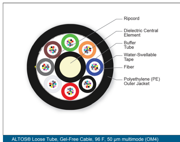
ALTOS® Loose Tube, Gel-Free Cable, 96 F, 50 µm multimode (OM4)
